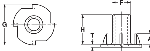
4-PRONG
