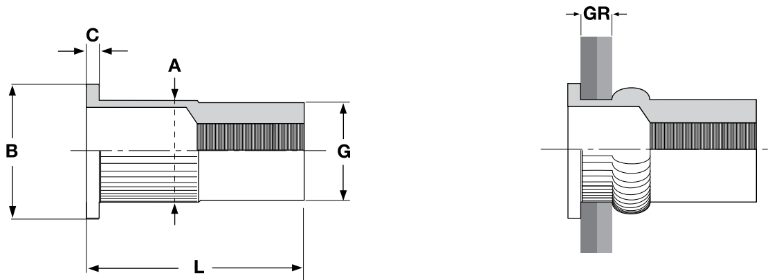
RIBBED BODY, FLAT HEAD, LARGE FLANGE BLIND THREADED INSERTS
